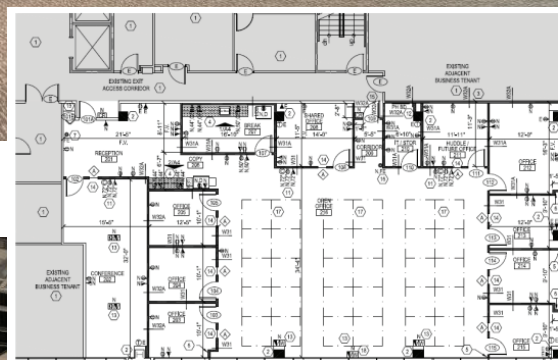
➡ 2 NEW CONSTRUCTION FLOOR PLAN SCALE: 1/8"=1'-0"
